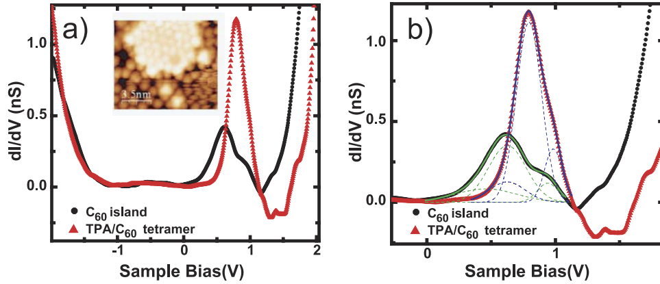
Figure 8. (a) dI/dV-V curves ( V_{ac} = 7 mV rms , V = 2.3 V, I = 1.1 nA) recorded on a TPA/ C_{60} tetramer (red, triangles) and on a pure C_{60} island (black, circles) (see inset). The LUMO of C_{60} in the islands is found at \sim 630 meV with an overall width of \sim 480 meV, while the C_{60} in the tetramers exhibits the LUMO with negative differential resistance (NDR) at \sim 810 meV with a smaller width of \sim 290 meV. (b) The LUMO lineshapes are fitted by three Gaussians (dashed lines). In a pure C_{60} island these are centered at 460, 640, and 940 meV with FWHM of 480, 300, and 160 meV, respectively. A smaller splitting (Gaussians centered at 630, 800, and 990 meV) and smaller FWHM (280, 200, and 140 meV) are found in the C_{60} in the tetramers.
